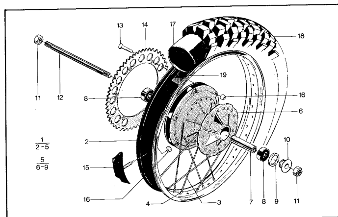
Bakhjul. Rearwheel.
