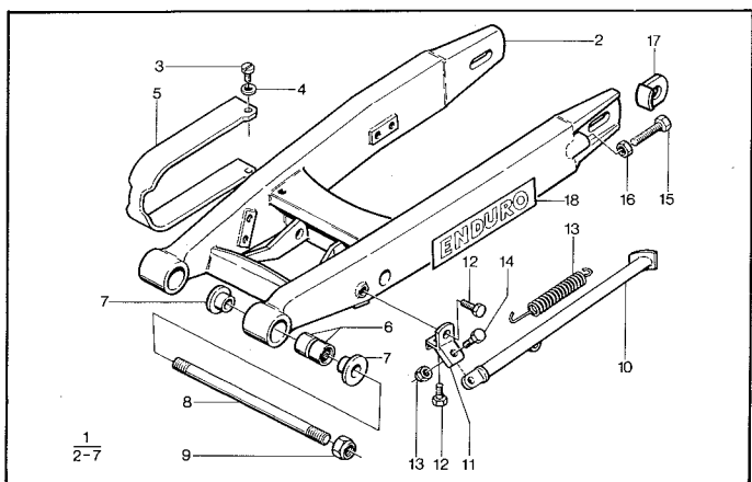
Sving. Swingarm.
