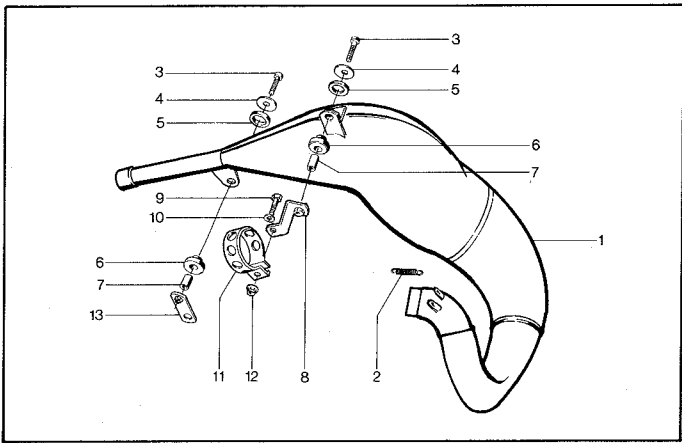
Avgasrör. Exhaustpipe.
