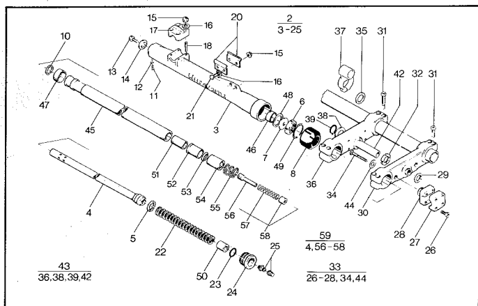
Framgaffel. Frontfork.
