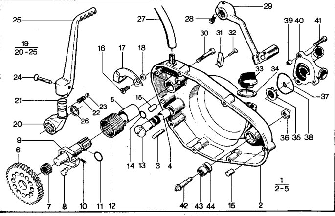
Transmissionskåpa. Transmissioncover.
