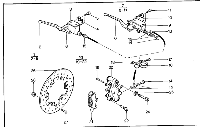
Frambroms. Frontbrake.
