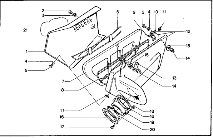
Luftburk. Airfilterbox.
