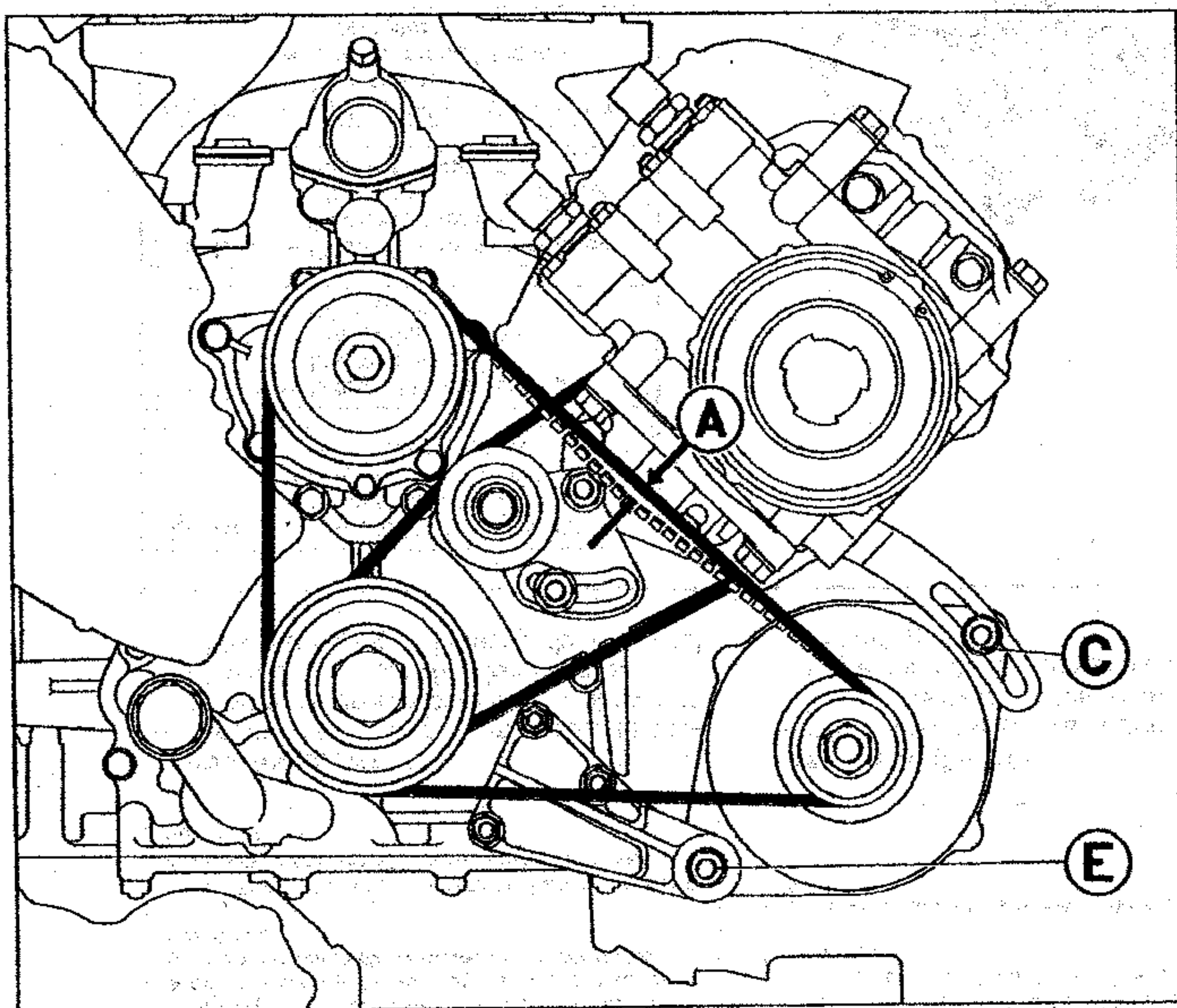
Fig. 11 = Belt tension of water pump drive (308)
