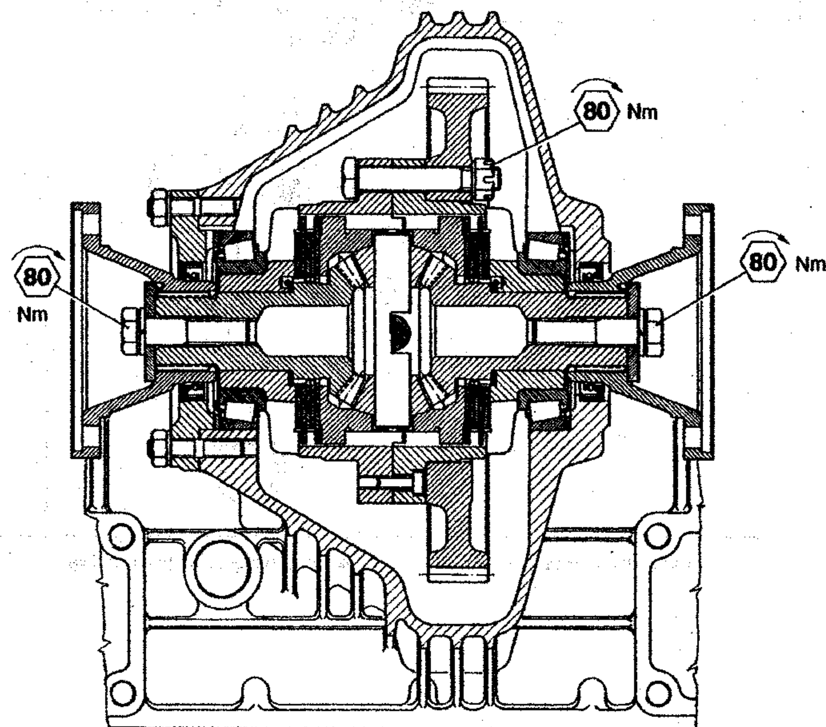
Fig.19 = Plate-type limited-slip differential
