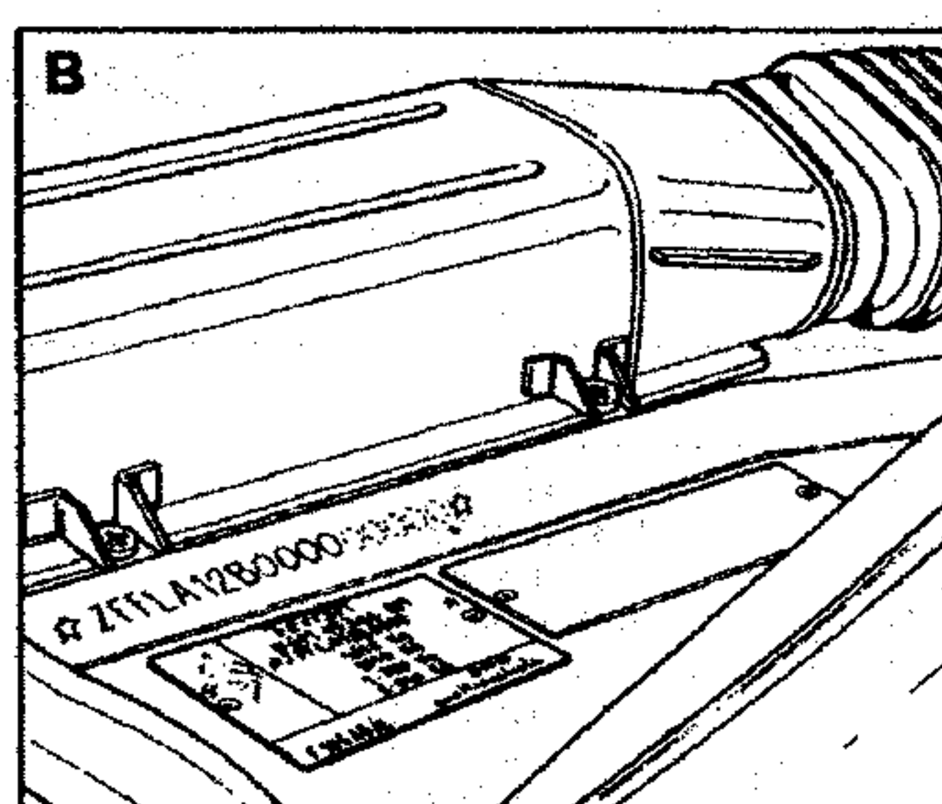
Fig. 3 = Identification Data 308
